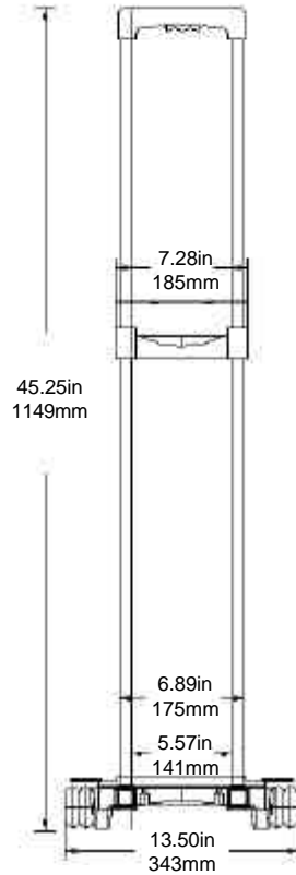
Front View
