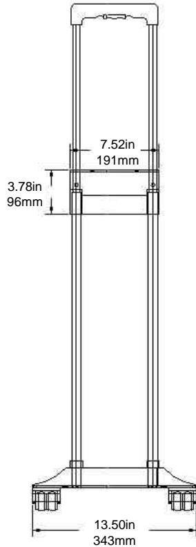
Front View
